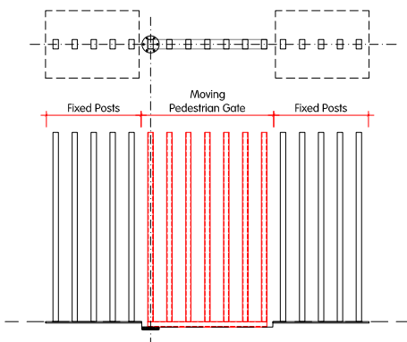
Level Surface
