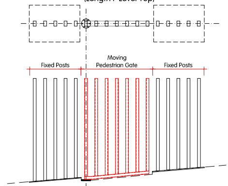
Sloped Surface
